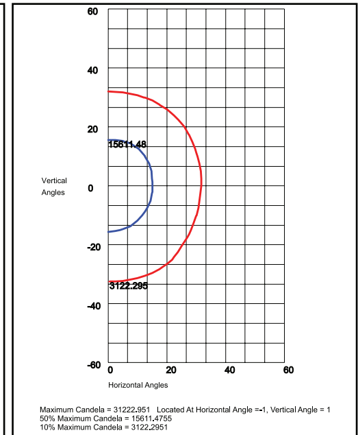
PKH25QI1X112U5KC 30°H x 30°V, NEMA 4H x 4V
